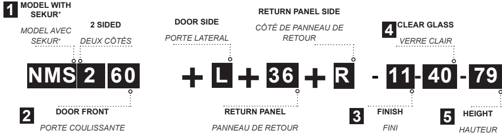
IN-LINE RIGHT INNER DOOR CLOSING WITH WALL WITH RETURN PANEL ON RIGHT SIDE
