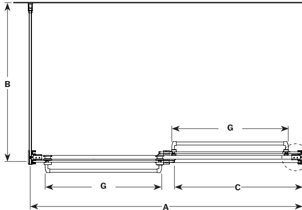
Top view / Plan
