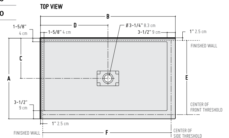
Right-side tile flange configuration
