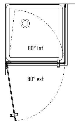
TOP VIEW • TJCR3336
