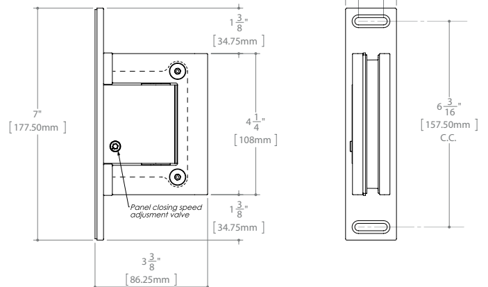
BACK VIEW
