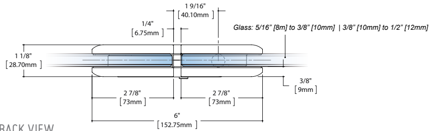
BACK VIEW
