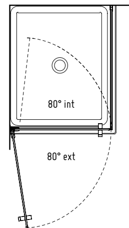
TOP VIEW • TJCR3348
