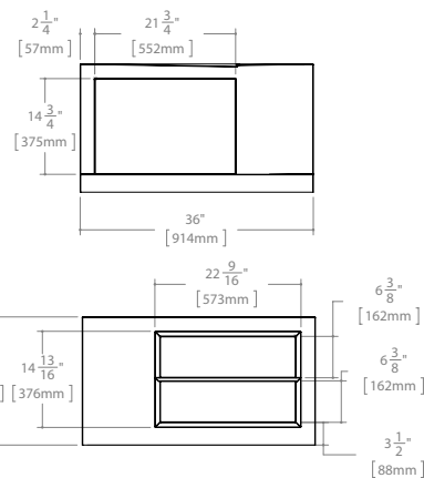
Left-side configuration BSSU3660L-18W
