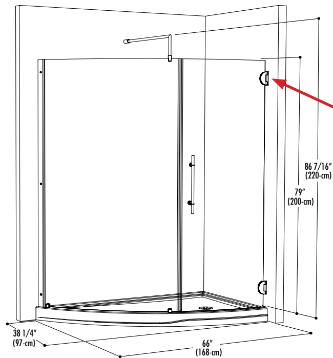
Left-side configuration
