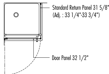
TOP VIEW • PXQ3636
