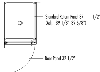
TOP VIEW • PXQ3642
