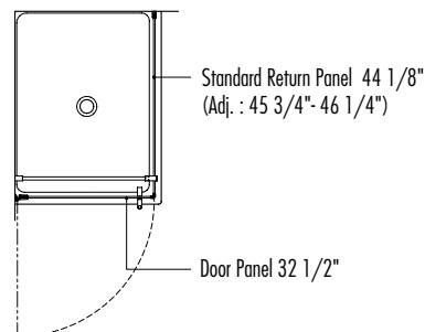
TOP VIEW • PXQ3648
