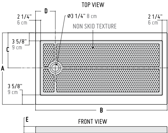
ABF3260** Side Drain Acrylic Base
