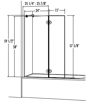
Support Bar System
