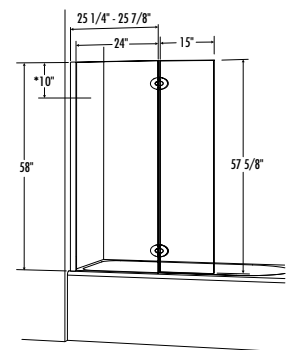
Glass Shelf Support
