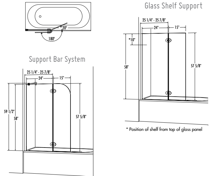
SUPPORT BAR SYSTEM - "X"
