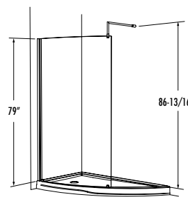
ABSL66-18L Flanged Slice, End Drain Left Side Configuration
