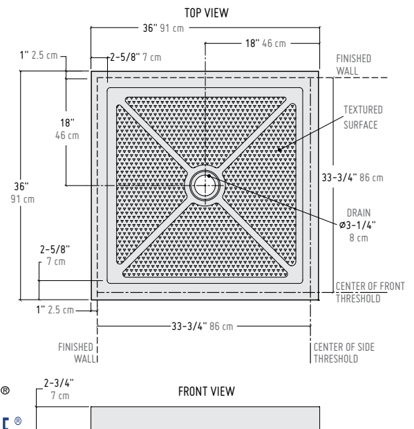
BASE ABF3636
