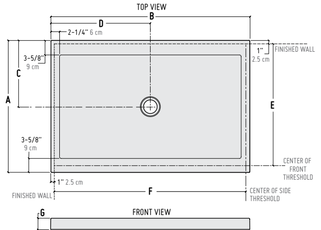
BASE ABF3636
